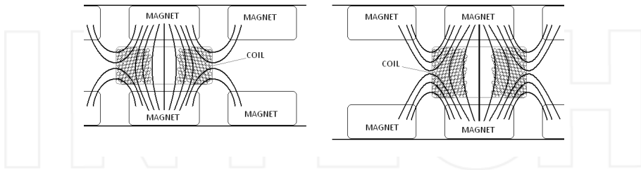
Figure 7. Lateral flux short circuiting to adjacent magnets increases (right) with increased rotor separation distance.
